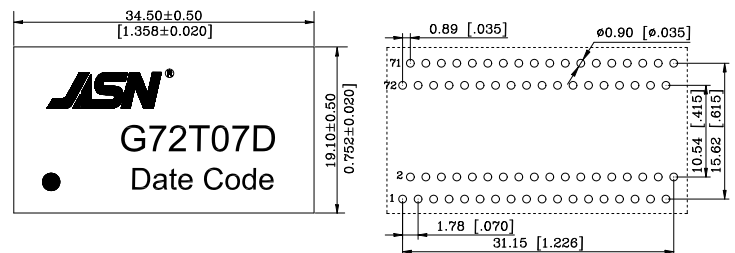
SUGGESTED PCB LAYOUT
